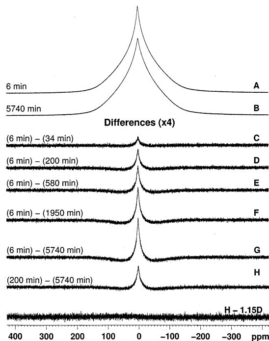
Figure 3. Bloch-decay spectra and difference spectra associated with a 4 d aging period for iPP-1. A, B: full spectra for t_{\text{age}} = 6 min and 4 d, respectively. C–H: vertically amplified ( \times 4 ), zero-integral difference spectra involving spectra at the 2 indicated t_{\text{age}} values. Spectrum G = A – B. The lower spectrum is the indicated “difference of difference” spectrum illustrating that, within experimental error, the line shape changes over the first half of the aging-induced conversion are identical to those in the second half.
