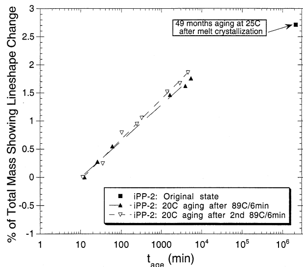
Figure 6. Plot, similar to Figure 5, for the metallocene polymerized iPP-2. Note that the thermal treatments are duplicated here and that the starting points are identical, indicating that a repetition of the heating cycle destroys all of the aging-induced structures formed after the first heating cycle.
