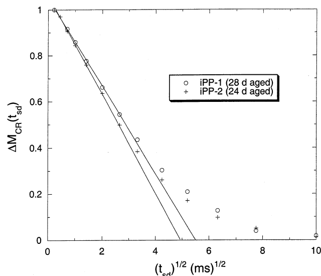
Figure 10. Spin diffusion plots for similarly aged iPP-1 and iPP-2 based on nonspinning T_{1xz} – T_{1xz} –SD experiments using variable spin diffusion times, t_{sd} . The preparation is the selection of crystalline magnetization using 16 ms of T_{1xz} . The ordinate measures the relative decrease in the CR magnetization vs t_{sd}^{0.5} with unity representing the CR magnetization at very short SD times and zero representing the CR magnetization when the polarization of all regions is equal (internal spin equilibrium). Straight lines are drawn to indicate initial slopes. The intercepts of these lines with the abscissa give characteristic times which can be used, in conjunction with crystallinity values, to estimate long periods (23 nm for iPP-2 and 24 nm for iPP-1). Thus, morphologies of iPP-1 and iPP-2, by this measure, are very similar. Also, the slope linearity at short times indicates that in the CR regions, all protons, including the methyl protons, have very long T_{1xz} 's.
