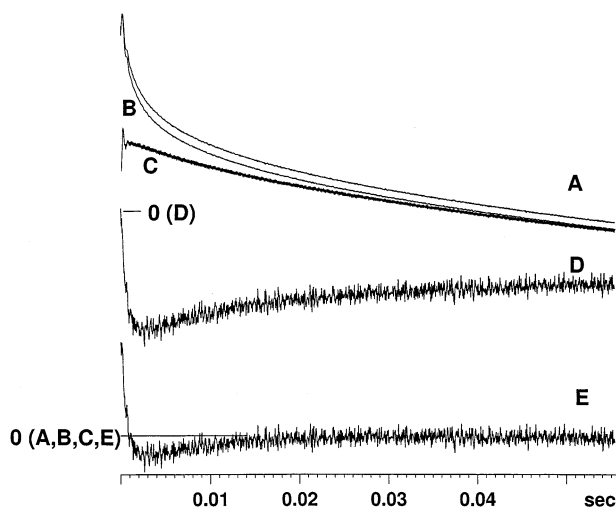
Figure 8. T_{1\rho} decays and decay differences for the nonspinning iPP-2 sample with different aging histories. A: T_{1\rho} for original sample, aged at 25 °C for 49 months. B: T_{1\rho} for same sample 30 min after a heating cycle to 89 °C for 6 min. C: Rescaled decay for the "B" sample using the T_{1\rho} - T_{1\rho} -SD experiment (16 ms of T_{1\rho} preparation, short spin diffusion time = 20 \mu\text{s} ). This experiment extracts the decay of the crystalline protons only. Rescaling is done to match the long-term decay of B. The ratio of initial intensities of C to B gives crystallinity ( 0.72 \pm 0.03 ) and the difference, B - C (not shown) gives the T_{1\rho} profile of the noncrystalline (NC) region. This NC decay is not single-exponential; instead, it can be broken down into one component with a T_{1\rho} of 1 ms, 0.19 \pm 0.02\% and another component with a T_{1\rho} in the 5–8 ms range, 0.09 \pm 0.02\% . The amplitude of the 1 ms component corresponds closely to the fraction of motionally averaged protons identified in the Bloch-decay spectrum. D = (A - B) \times 10 . This normalized difference starts at zero and goes quickly negative, indicating that B has a larger component with fast decay. The longer-time positive growth of D is truncated and indicates the presence of a long- T_{1\rho} component, present in A, which the subsequent heating has destroyed. E is the difference, D, with a scaled fraction of C added so as to null the long- T_{1\rho} component. Here one can more easily see that heating to 89 °C for 6 min has created an increase in the fastest- T_{1\rho} component, and that this increase arises mainly 75–80% from the longest- T_{1\rho} component and secondarily 20–25% from the intermediate- T_{1\rho} component. Note the "zero" levels indicated for each curve.
