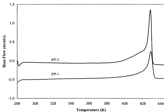
Figure 1. DSC heating traces showing crystalline melting endotherms. Endotherms are different in size because the iPP-2 sample size is about 50% larger than for iPP-1; moreover, the crystallinity of the former is higher.
