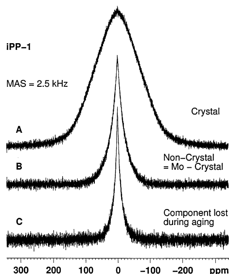
Figure 9. Different Bloch-decay line shape components for the iPP-1 sample at \nu_r = 2.5 kHz. A: crystalline line shape from the T_{1\rho} -FID-SD experiment with a 16 ms T_{1\rho} preparation and a spin diffusion time of 20 \mu\text{s} . (This line shape also agrees very well with the line shape obtained using a nonspinning sample.) B: Spectrum of NC protons obtained by difference ( =M_0 - kA where k is chosen to be a maximum, subject to the condition that no negative intensity is allowed). C: Spectrum of the narrow component lost in the aging process (same as Figure 4C). That aging preferentially changes the population of the more mobile protons in the NC region is possibly an indication that secondary crystallization is happening in regions more distant from crystal surfaces.
