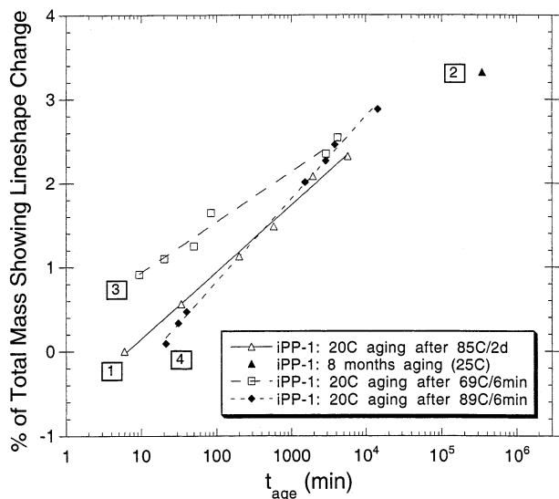
Figure 5. Percentages of the total mass showing line shape changes vs \log(t_{age}) at 20 °C for iPP-1, the Ziegler–Natta polymerized sample. The legends define the initial thermal treatment and the numbered boxes in the figure indicate the sequence of thermal treatments. Note especially the linearity of these plots and the fact that thermal cycling to 69 °C does not create as strong an initial mobile fraction as does the subsequent heating to 89 °C. The “zero” level in this plot is taken, arbitrarily, to be the condition at the time of earliest sampling after the first heating cycle. Note also that the point representing the 8-month aging period represents aging at 25 °C, not 20 °C. Estimated standard uncertainties associated with each datum in this and Figures 6 and 7 is \pm 0.15\% .
